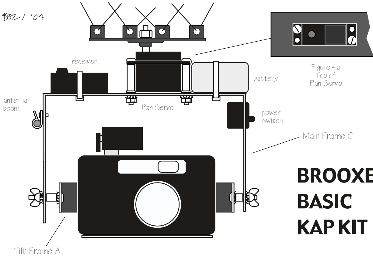
Figure 6 — Tilt Configuration
