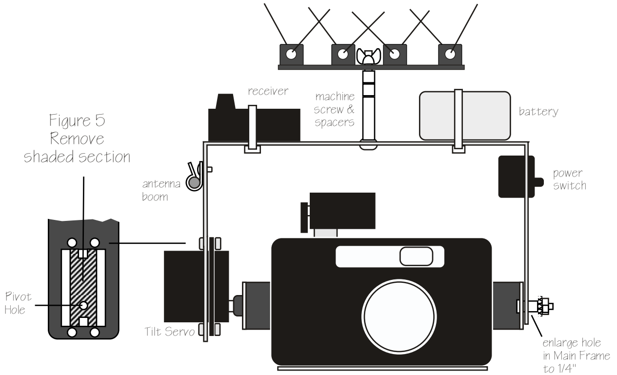
Figure 6 — Tilt Configuration
