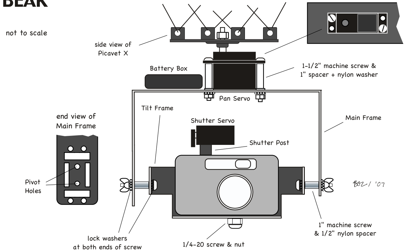
Figure 5A Top of Pan Servo
